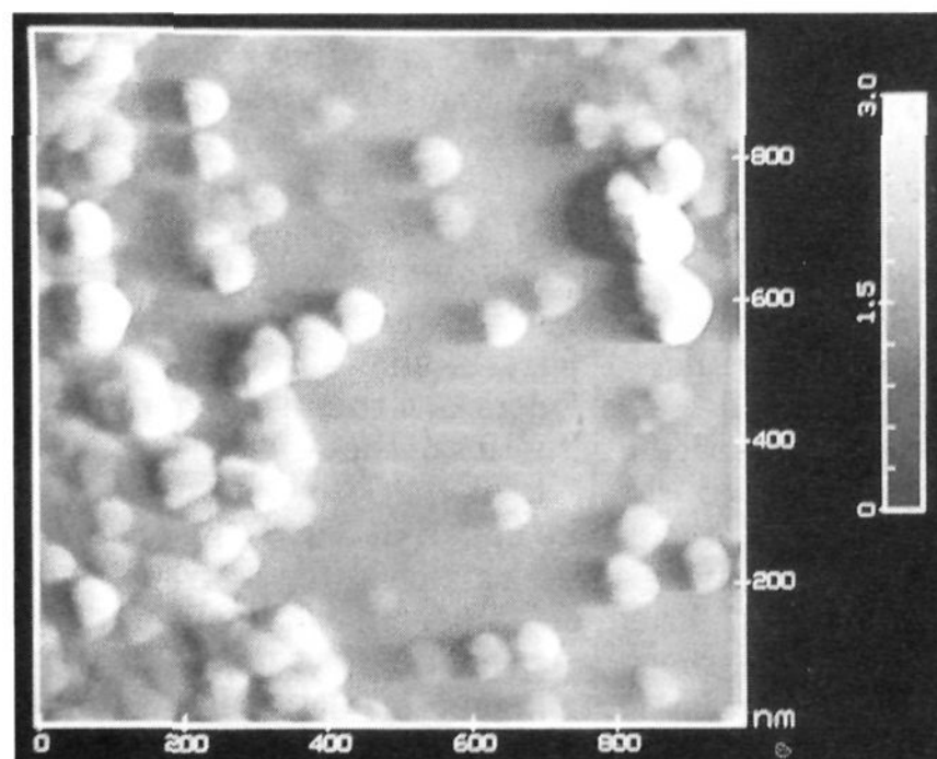
Figure 13. An atomic force micrograph of an \sim 10 \text{ nm} \text{SiO}_2 film on Mo(100) subsequent to the deposition of 10 monolayer equivalents of palladium and an anneal to 700 K.
