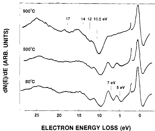
Figure 7. First-derivative electron energy loss spectra for a \sim 50 Å silicon dioxide film on Mo(110) annealed to 80, 500, and 900 °C. The resolution of the analyzer is \sim 0.6 eV.
