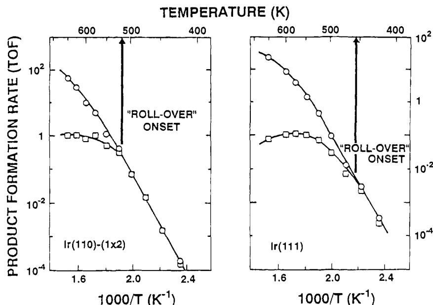
Figure 5. Arrhenius plot for propane hydrogenolysis reaction on Ir(110)-(1×2) and Ir(111) surfaces at a total reactant pressure P_T of 101 Torr and H_2/C_3H_8 = 100 : ○, methane; □, ethane.
